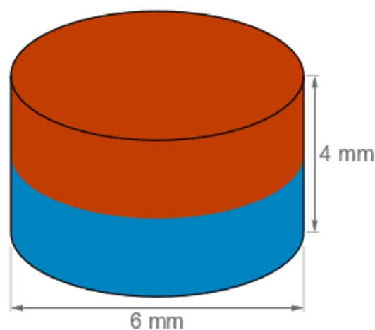
Dimensional drawing · all measurements in mm
