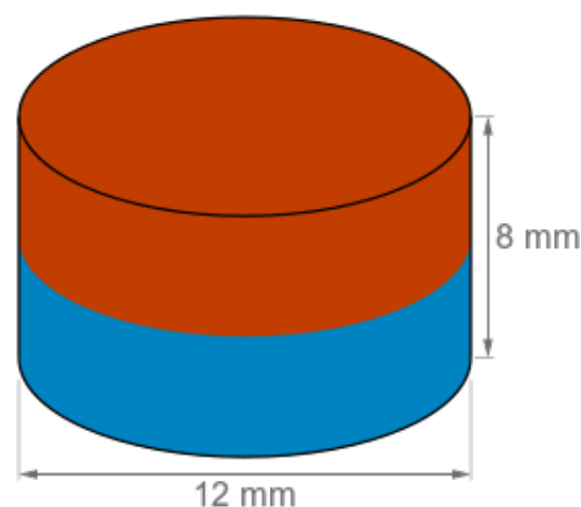
Dimensional drawing · all measurements in mm
