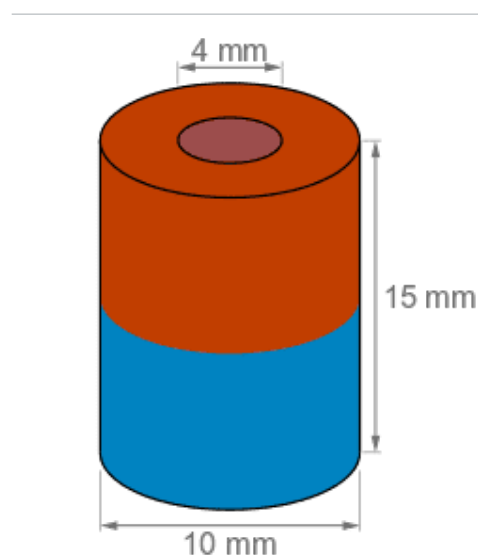
Dimensional drawing · all measurements in mm
