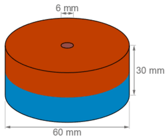
Dimensional drawing · all measurements in mm
