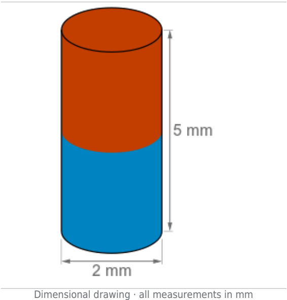
Dimensional drawing · all measurements in mm
